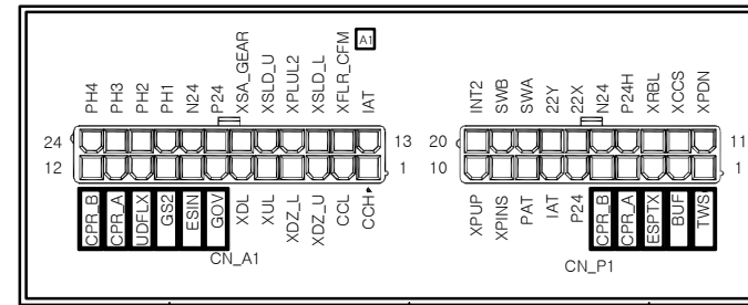
CPCON B'd(C/P) *BOARD TOP VIEW*
