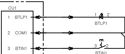
COP30D-N B'd (MAIN COP)
