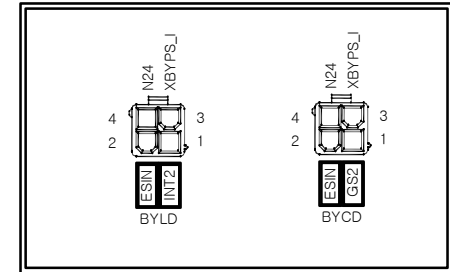
CPSW B'd(C/P) *BOARD TOP VIEW*
