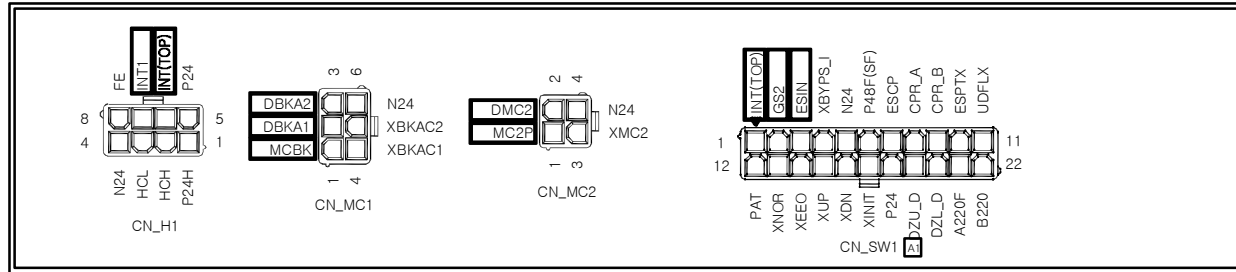
CPCON B'd(C/P) *BOARD TOP VIEW*
