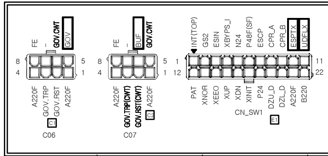
CPSW B'd(C/P) *BOARD TOP VIEW*
